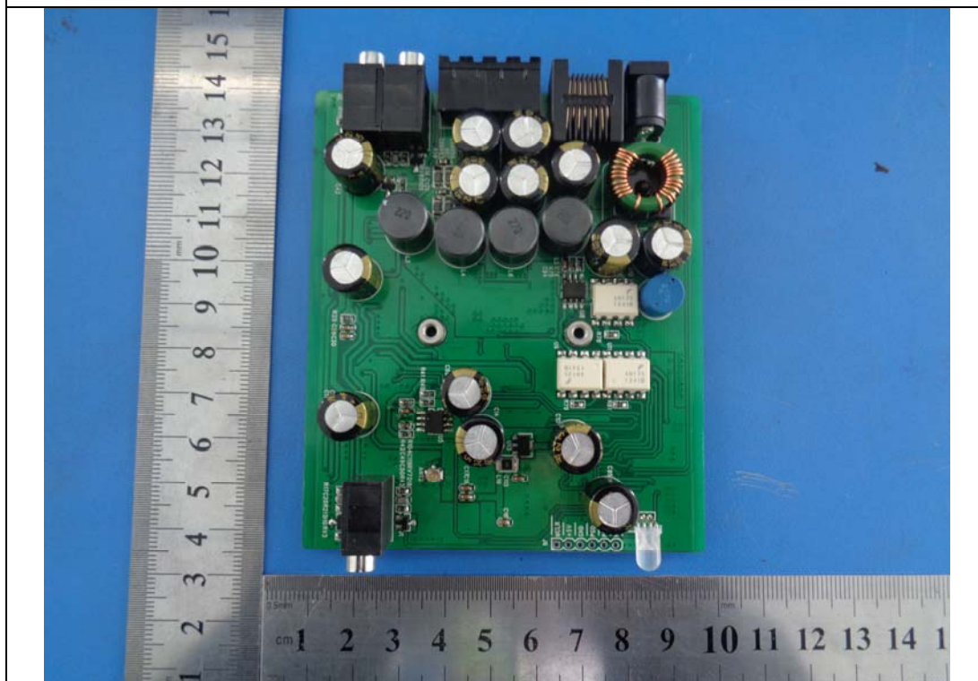
EUT – PCB Front View
