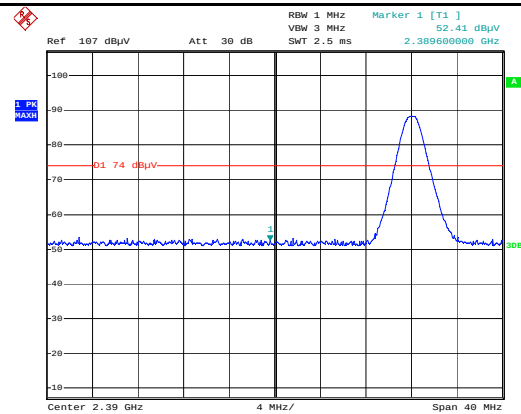
GFSK-Hopping-PK
