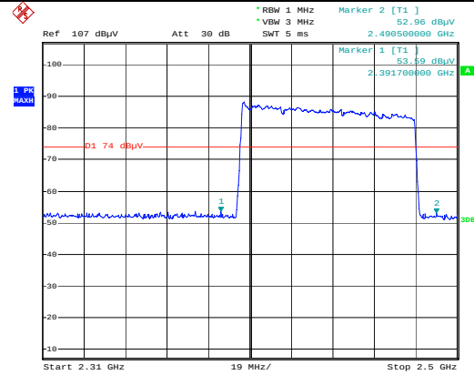
GFSK-Hopping-PK
