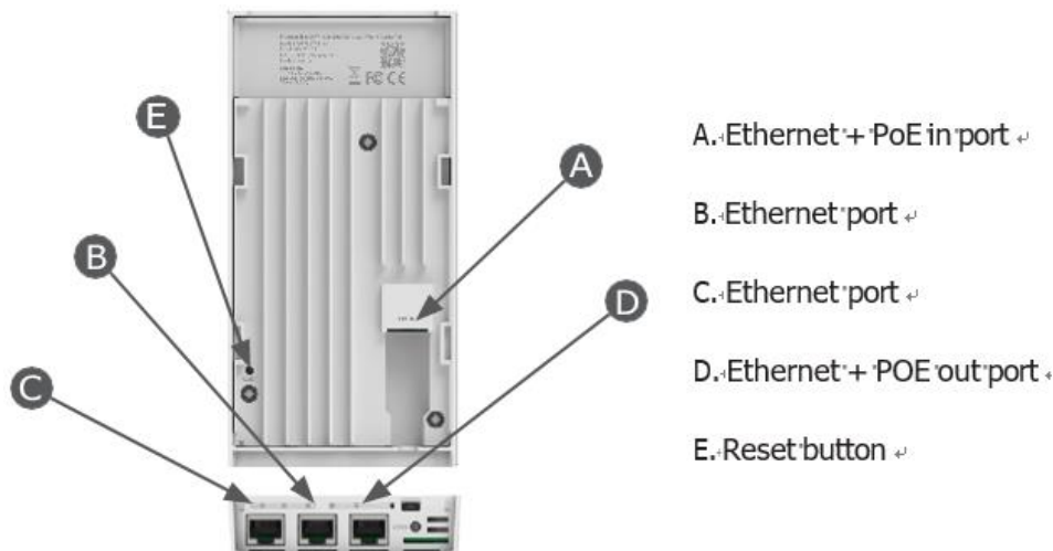
FIGURE 2: RAP750W-311A AP Ports on Bottom Panel.
