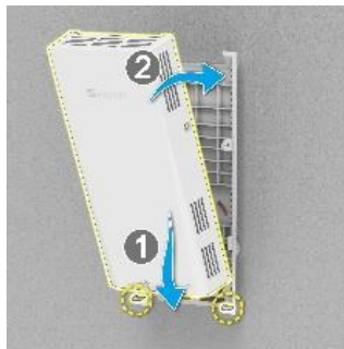
FIGURE 6: Fit into slots on the bottom of the RAP750W-311A
