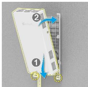
FIGURE 13: Fit into slots on the bottom of the RAP750W-311A
