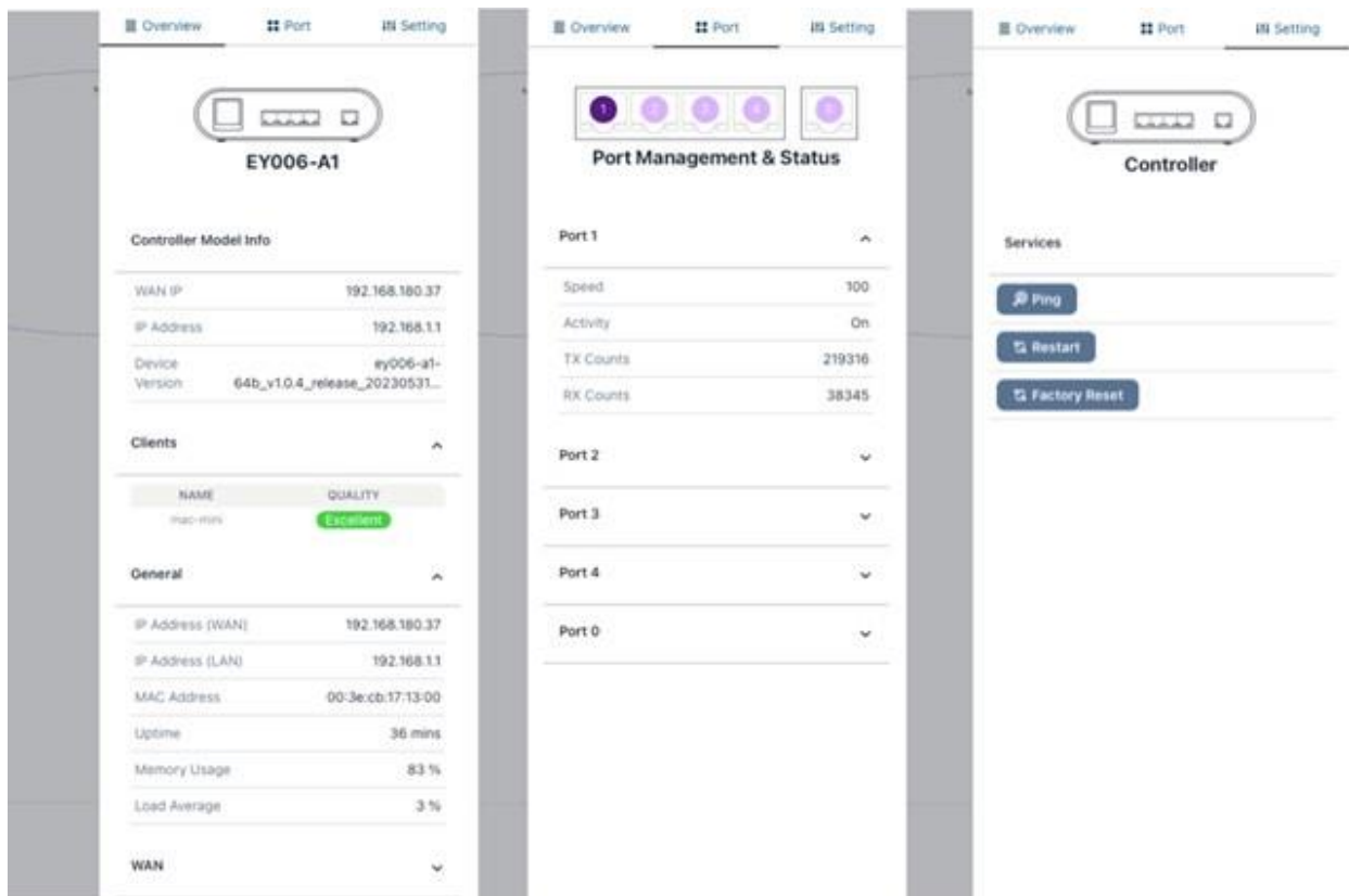
Figure 4. Controller Node Details
