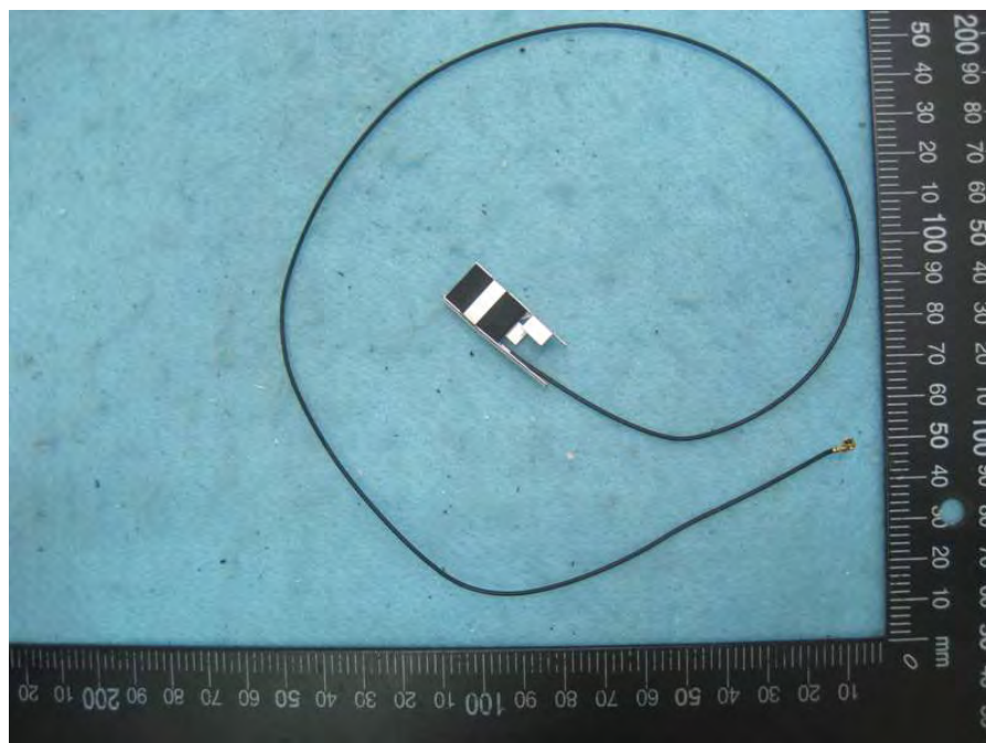
PIFA Antenna (Only for Bluetooth Function)
