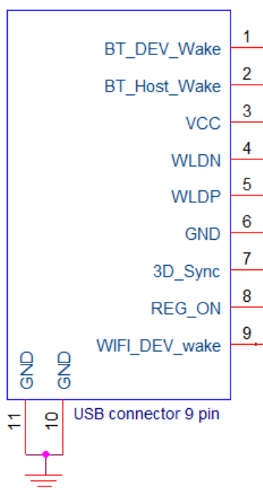
Figure 2: Pins Configuration
