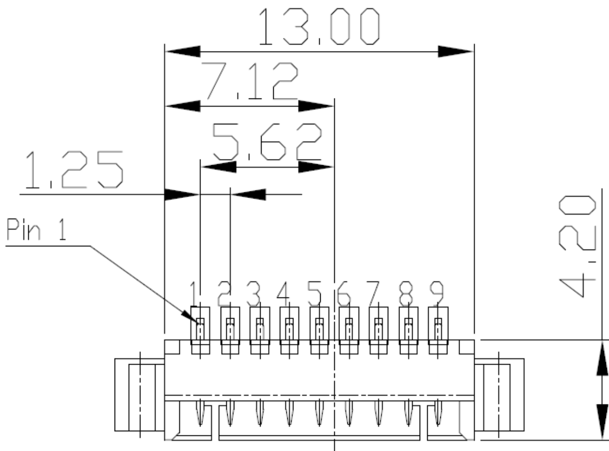
Figure 1: WTB Connector Layout
