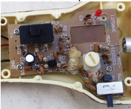
Inner Circuit Top View
