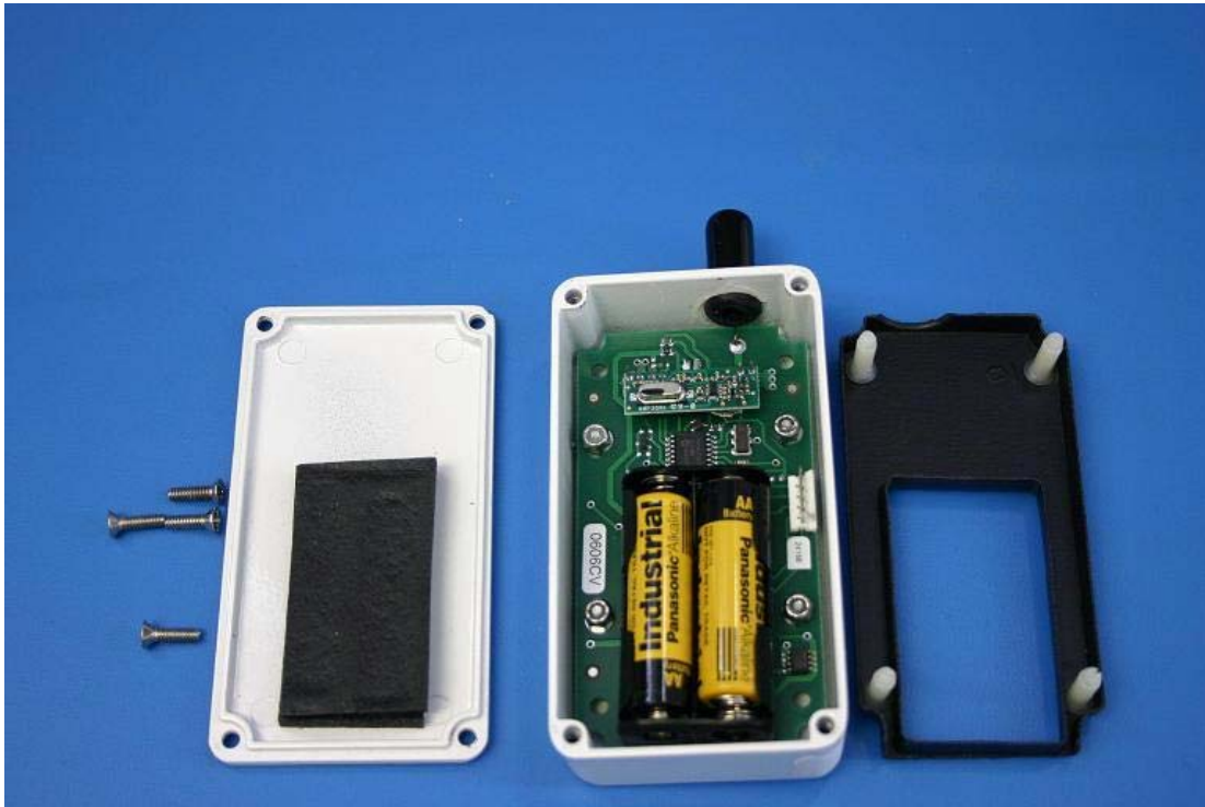
Figure 3: Eight Channel Transmitter With Exposed PCB
