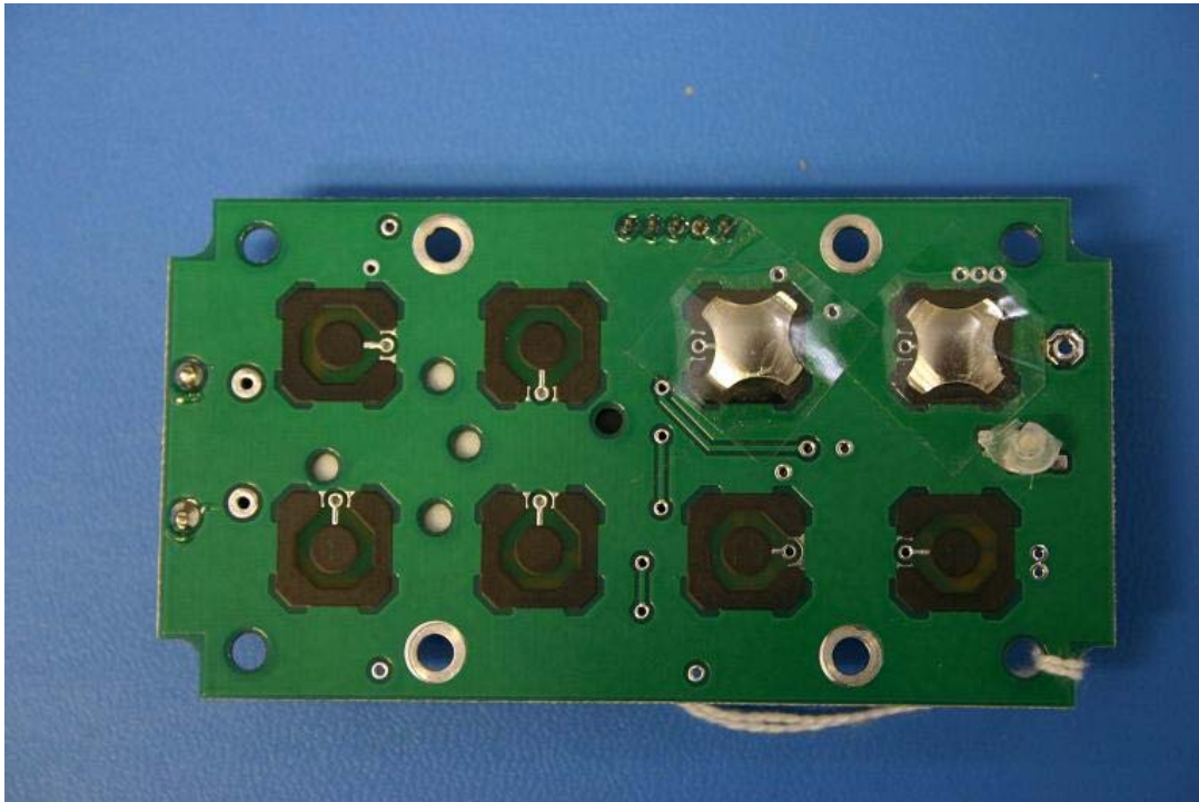
Figure 5: Switch / Bottom Side of PCB
