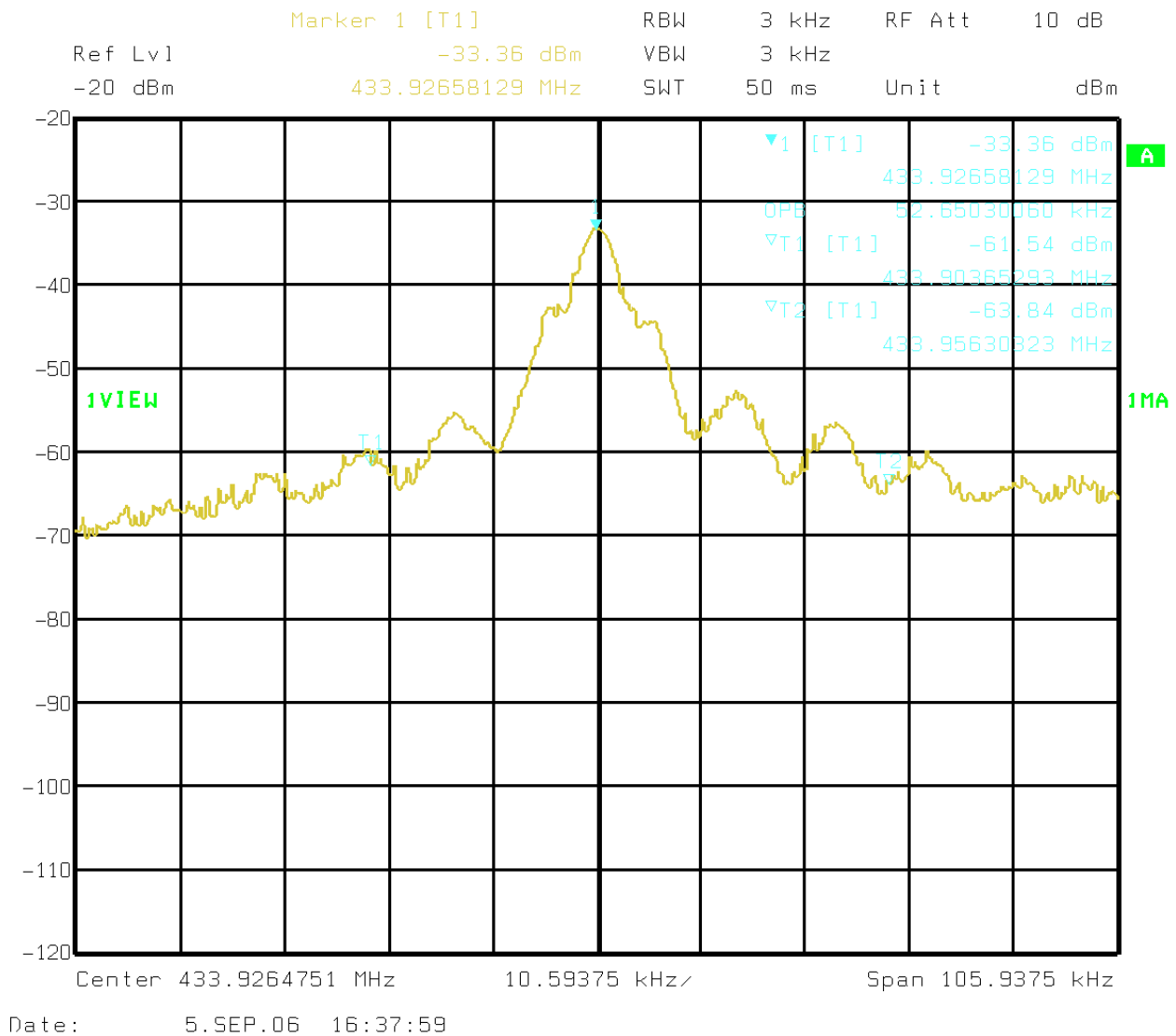
Figure 7-6: 2 99% Bandwidth
