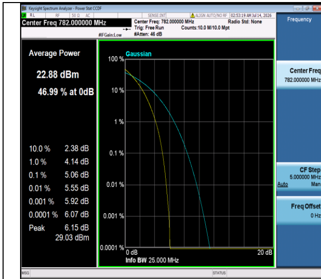
Band13-10MHz-QPSK-23230-50RB#0-PASS
