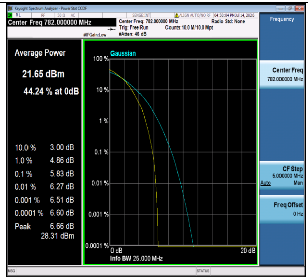
Band13-10MHz-16QAM-23230-27RB#0-PASS
