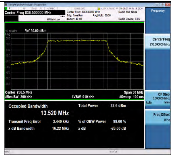
Band26(824-849)-15MHz-QPSK-26915-75RB#0-PASS
