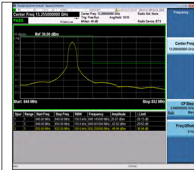
Band26(824-849)-15MHz-QPSK-26965-1RB#74-PASS
