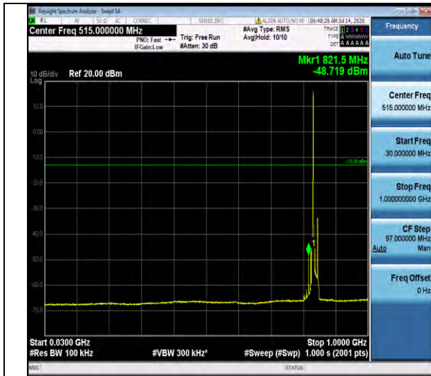
Band26(824-849)-15MHz-QPSK-26965-1RB#0-30~1000-PASS
