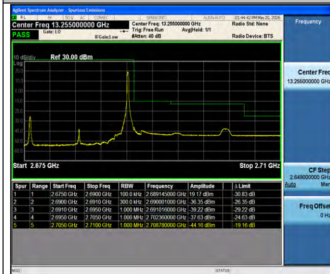
Band41-15MHz-QPSK-41515-1RB#74-PASS
