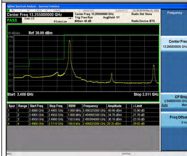
Band41-15MHz-QPSK-39725-1RB#0-PASS
