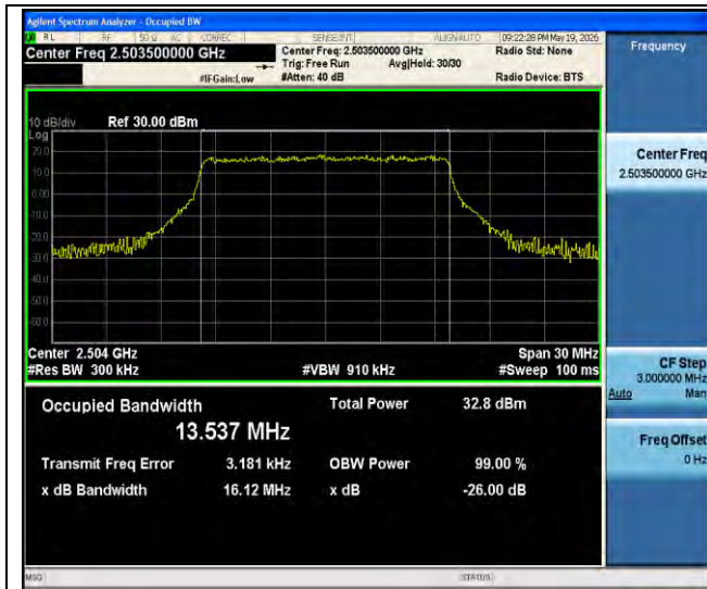
Band41-15MHz-QPSK-39725-75RB#0-PASS
