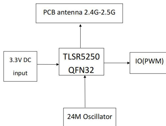
Picture 3-2 Internal block diagram of the E55 series module.
