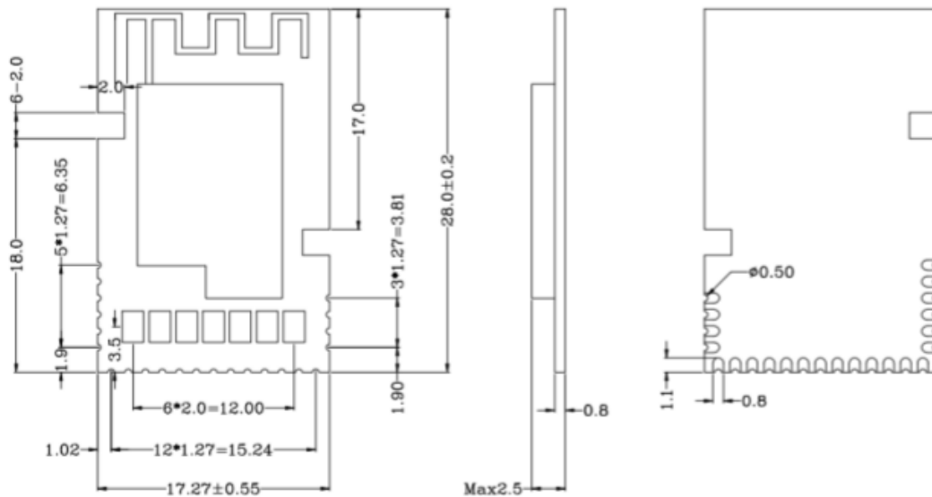
Drawing 2-1 Dimensional Drawing for LSD4RF0436-10D0 PCBA (Unit: mm)
