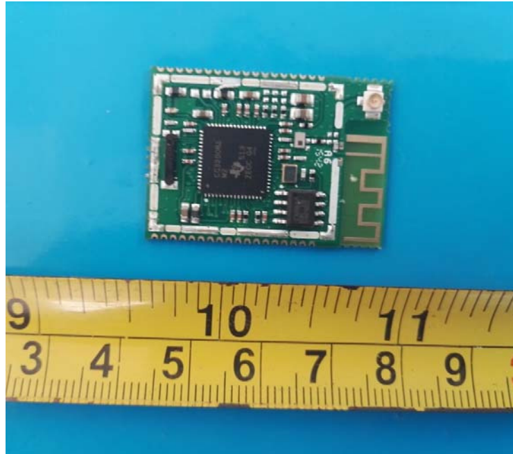
EUT –Shielding off View
