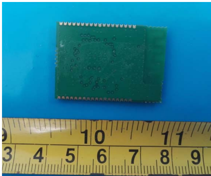
EUT – Main Board Bottom View
