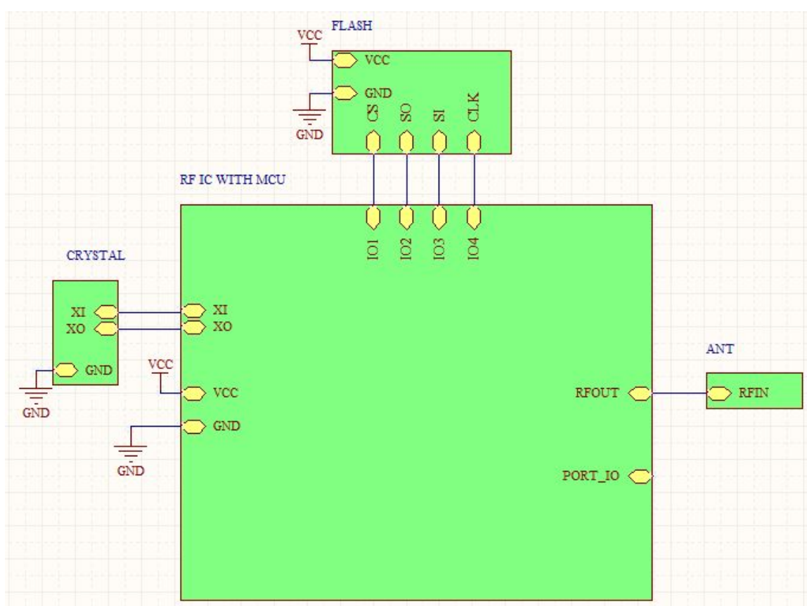
Figure 1 structure diagram
