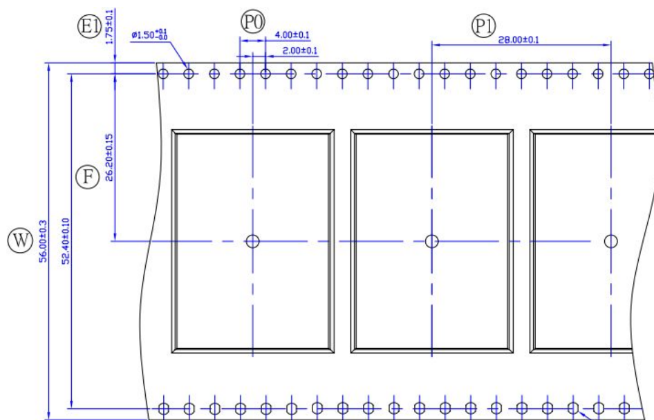
Figure 11 Tape size
