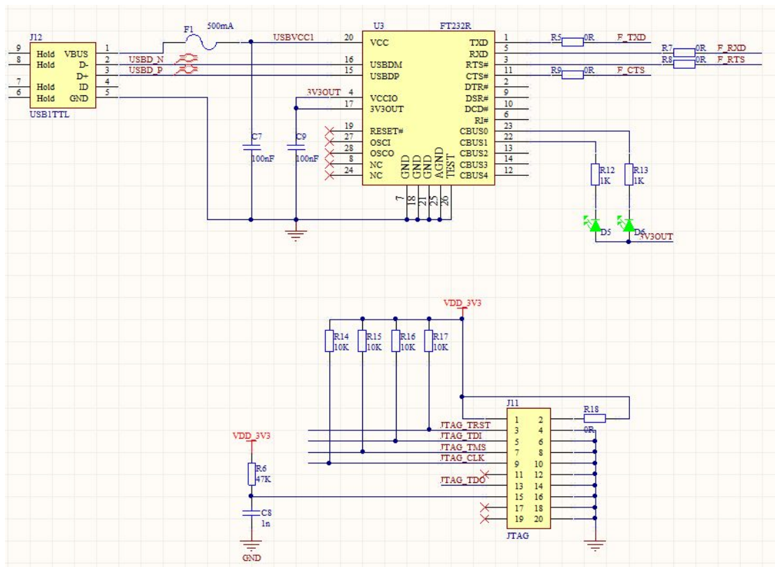
Figure 5 Reference design
