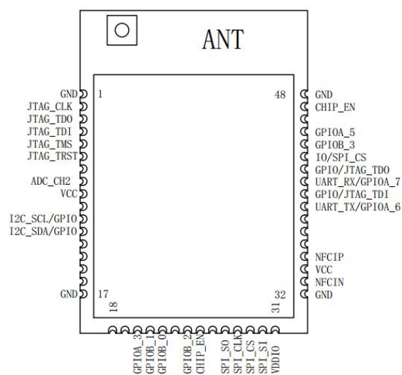
Figure 3 Module pin funtion diagram
