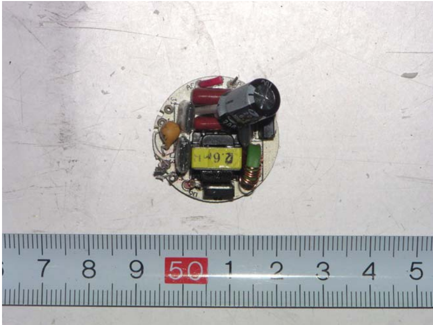
EB-7W-T2: PCB Front View
