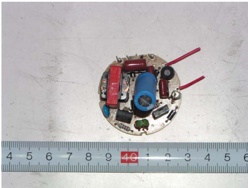
EU-25W-E26: PCB Front View
