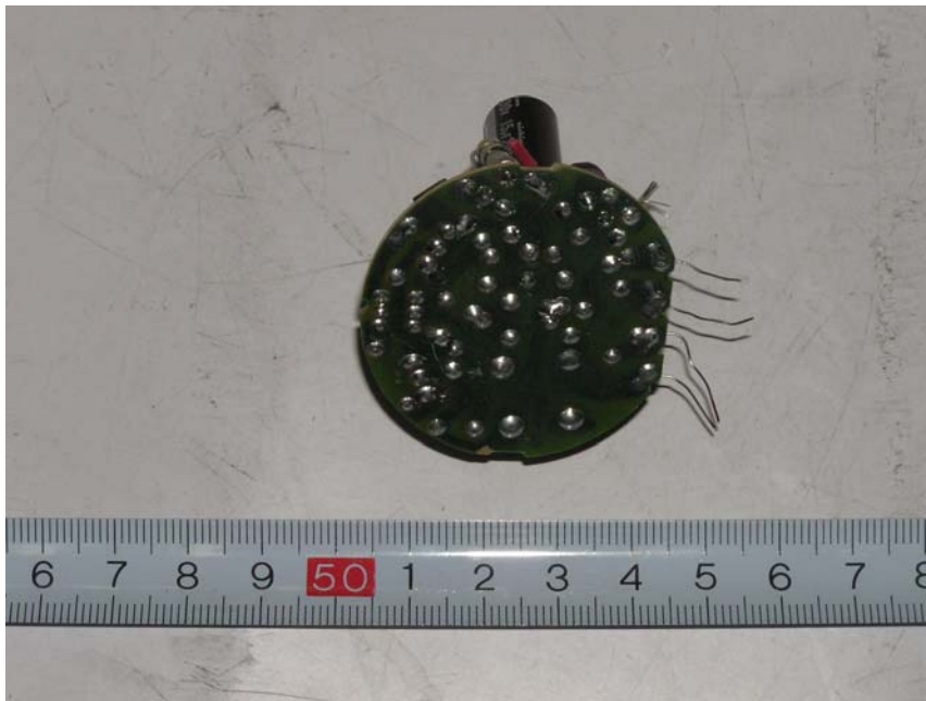
EU-25W-E26: Uncovered View
