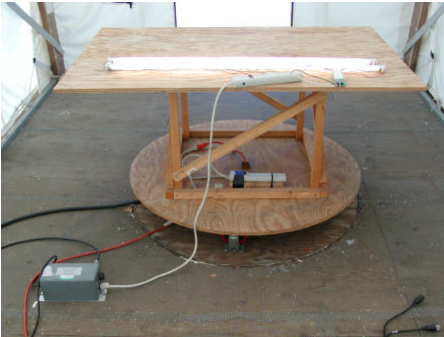
F32T8 Conducted Emission Photograph – Rear View
