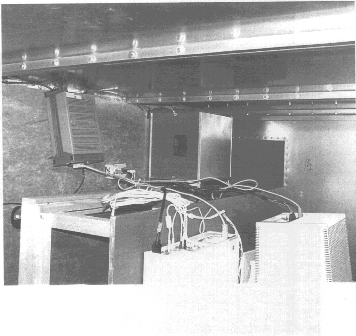
figure 4.2 conducted emission test setup
