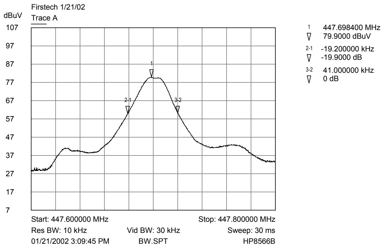
Bandwidth Plot
