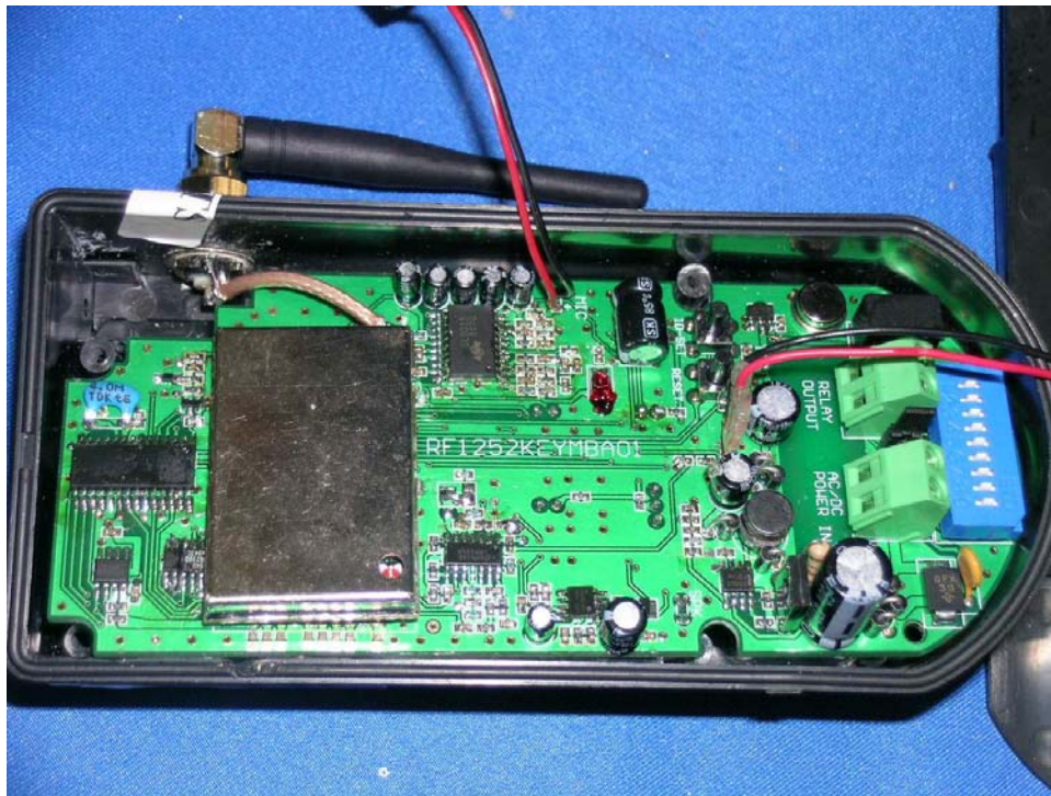
Keypad Main PCB comp side (View 1)
