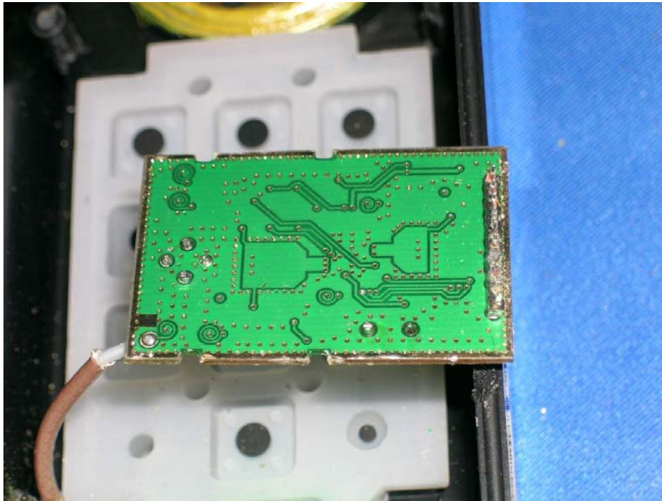
Keypad Oscillator PCB solder side
