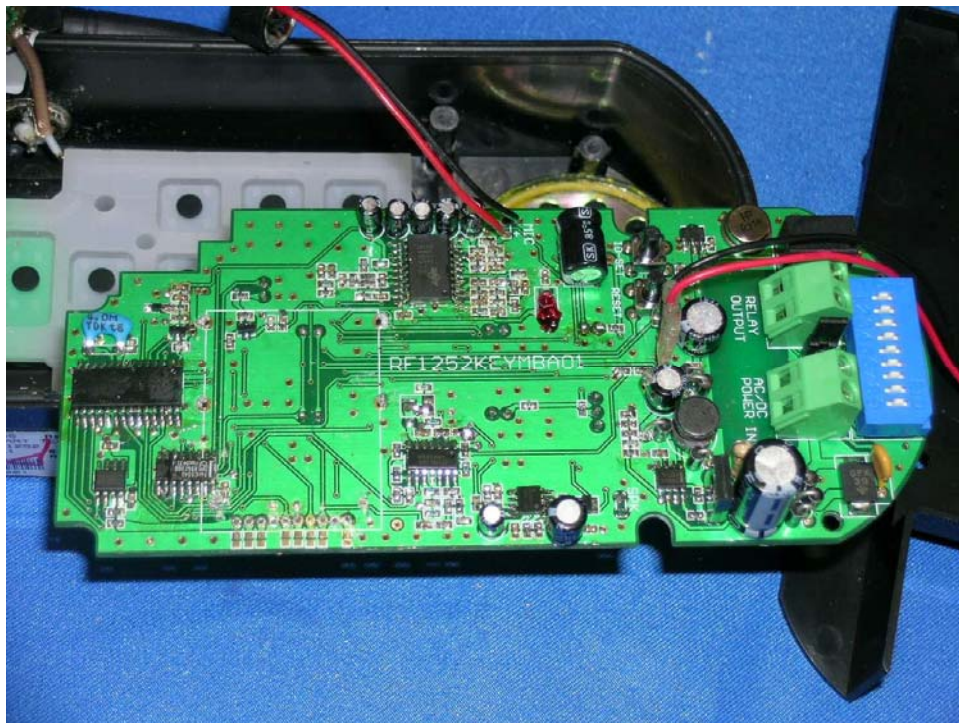
Keypad Main PCB comp side (View 2)
