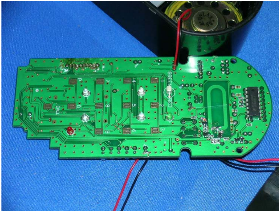
Keypad Main PCB solder side
