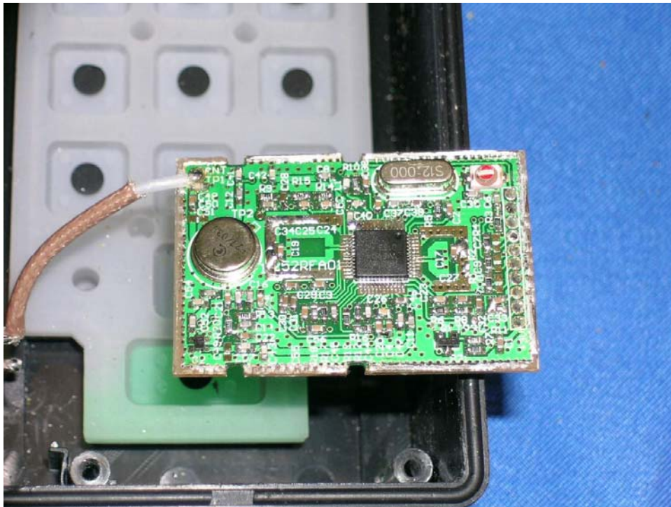
Keypad Oscillator PCB comp side
