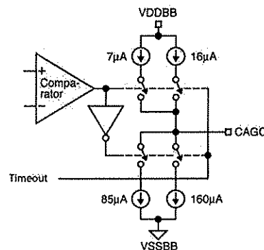
Figure 3. CAGC Pin
