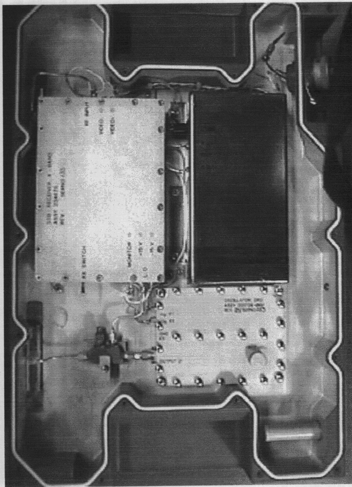
Photo 2: Internal construction
