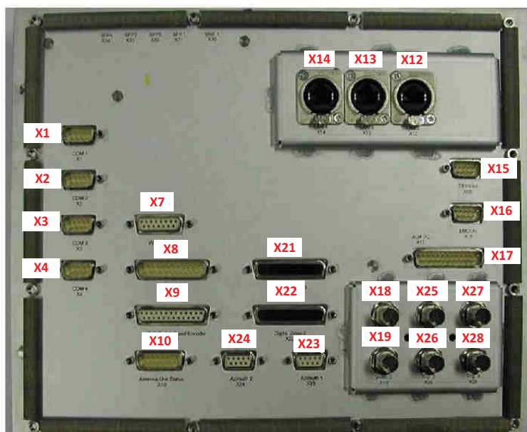
Fig. 5.27 External I/O, connections
