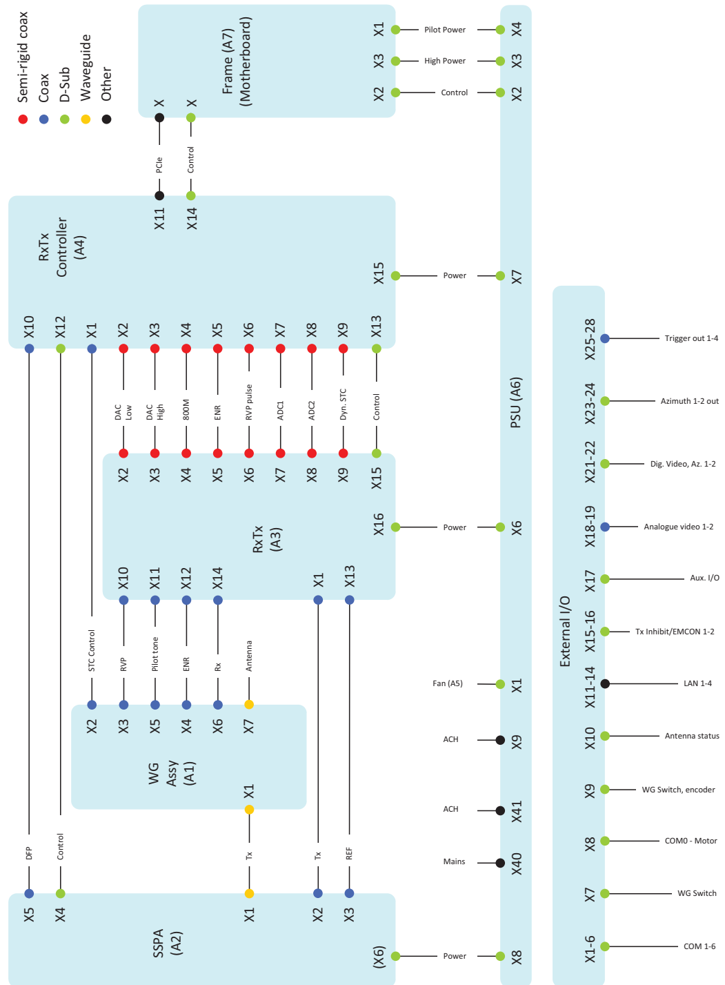
Fig. 5.4 Internal cabling
