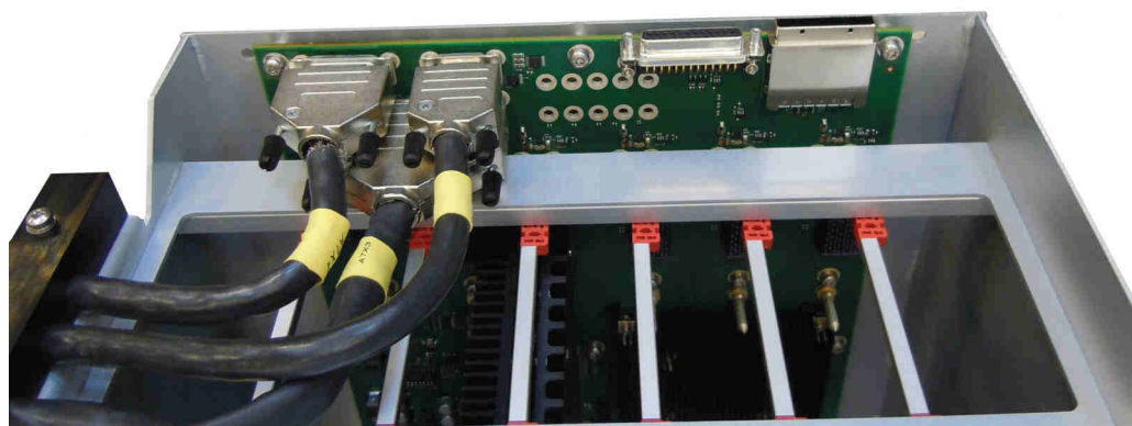
Fig. 5.17 Motherboard and connections shown in crate assy
