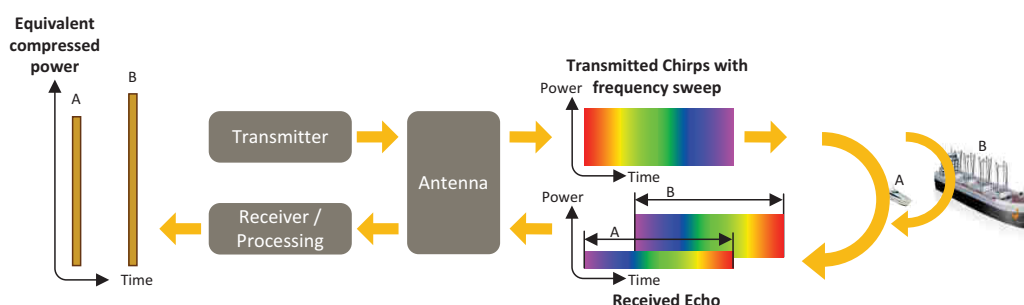
Fig. 3.8 Frequency sweep
