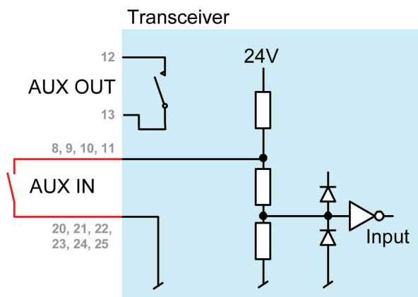
Fig. 5.33 Input circuit, AUX inputs/output
