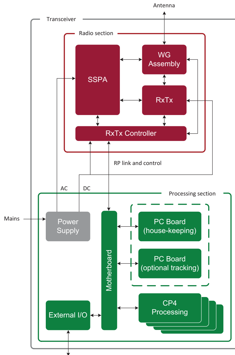
Fig. 4.2 Block schematic
