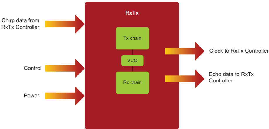
Fig. 4.12 Signal categories to and from RxTx
