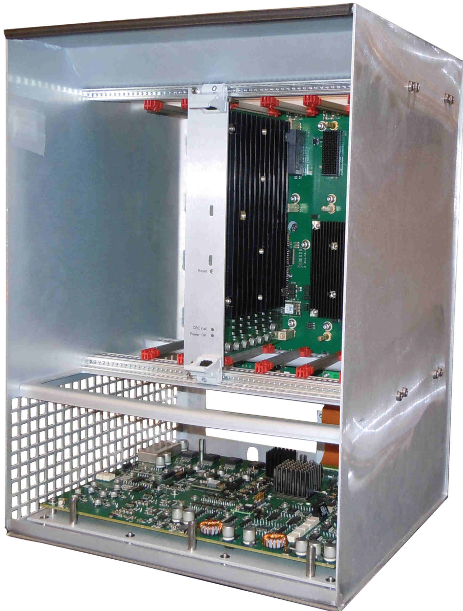
Fig. 4.16 Frame assy, shown with Ext. I/O and a CP4 board
