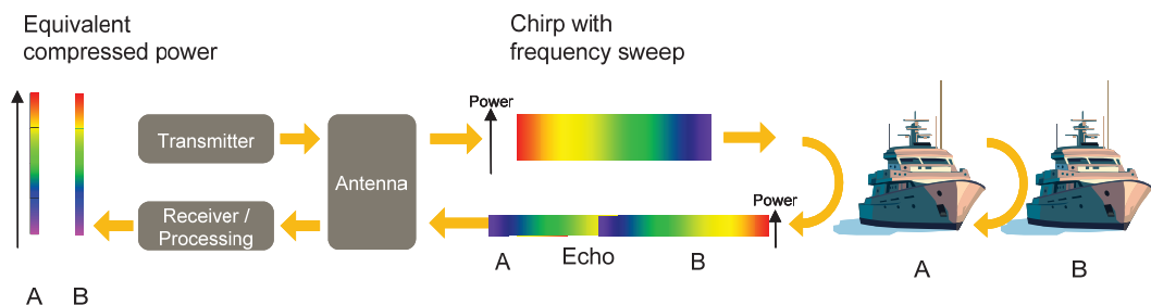
Fig. 3.6 Frequency sweep
