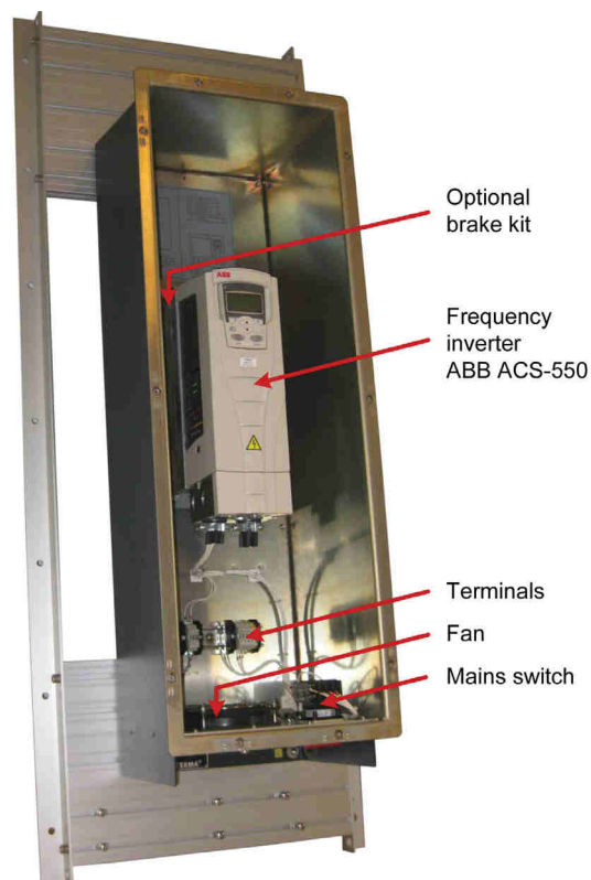
Fig. 4.37 Antenna Control Unit, open
