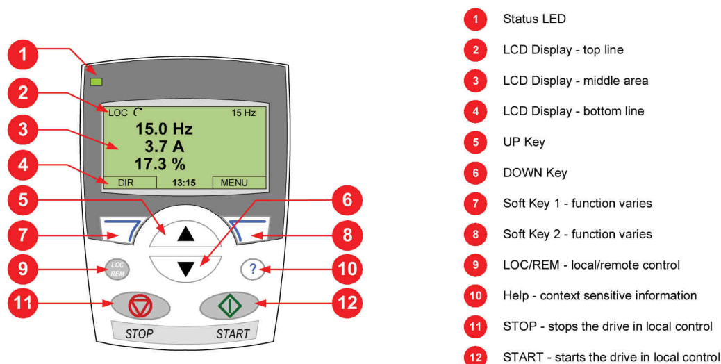
Fig. 4.41 Operator's panel
