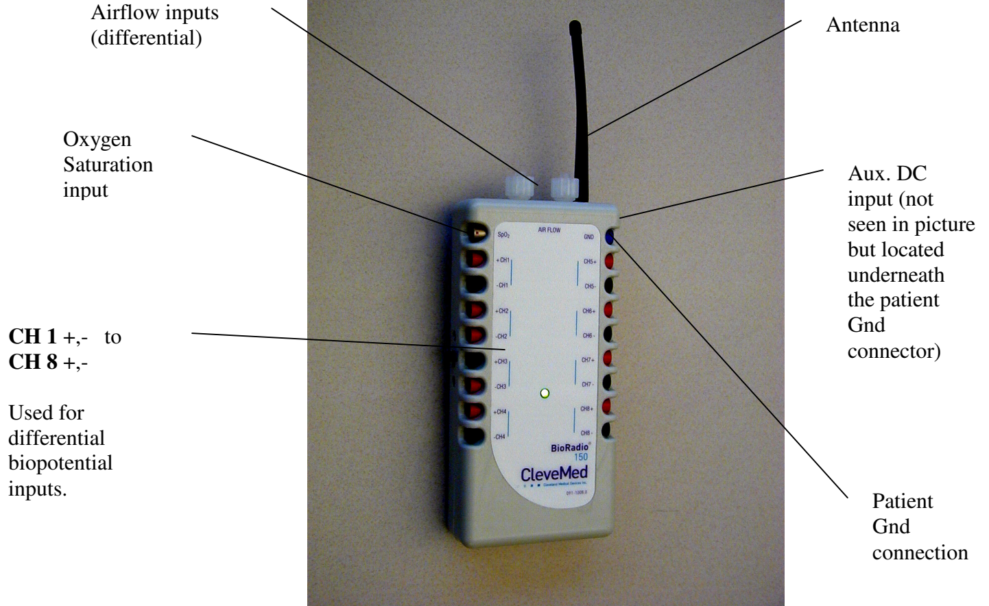
Figure 2. The BioRadio 150 User unit.
