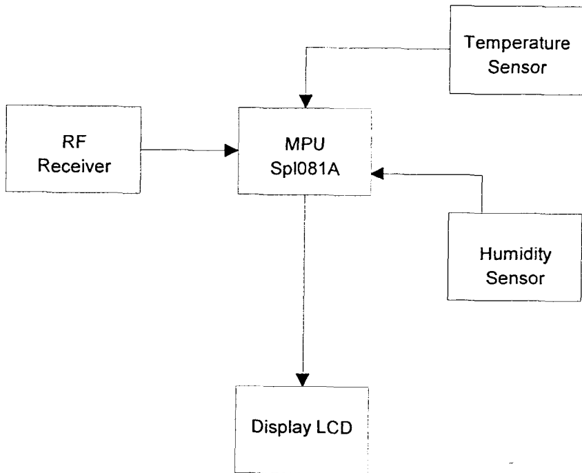
Receiver Block Diagram
