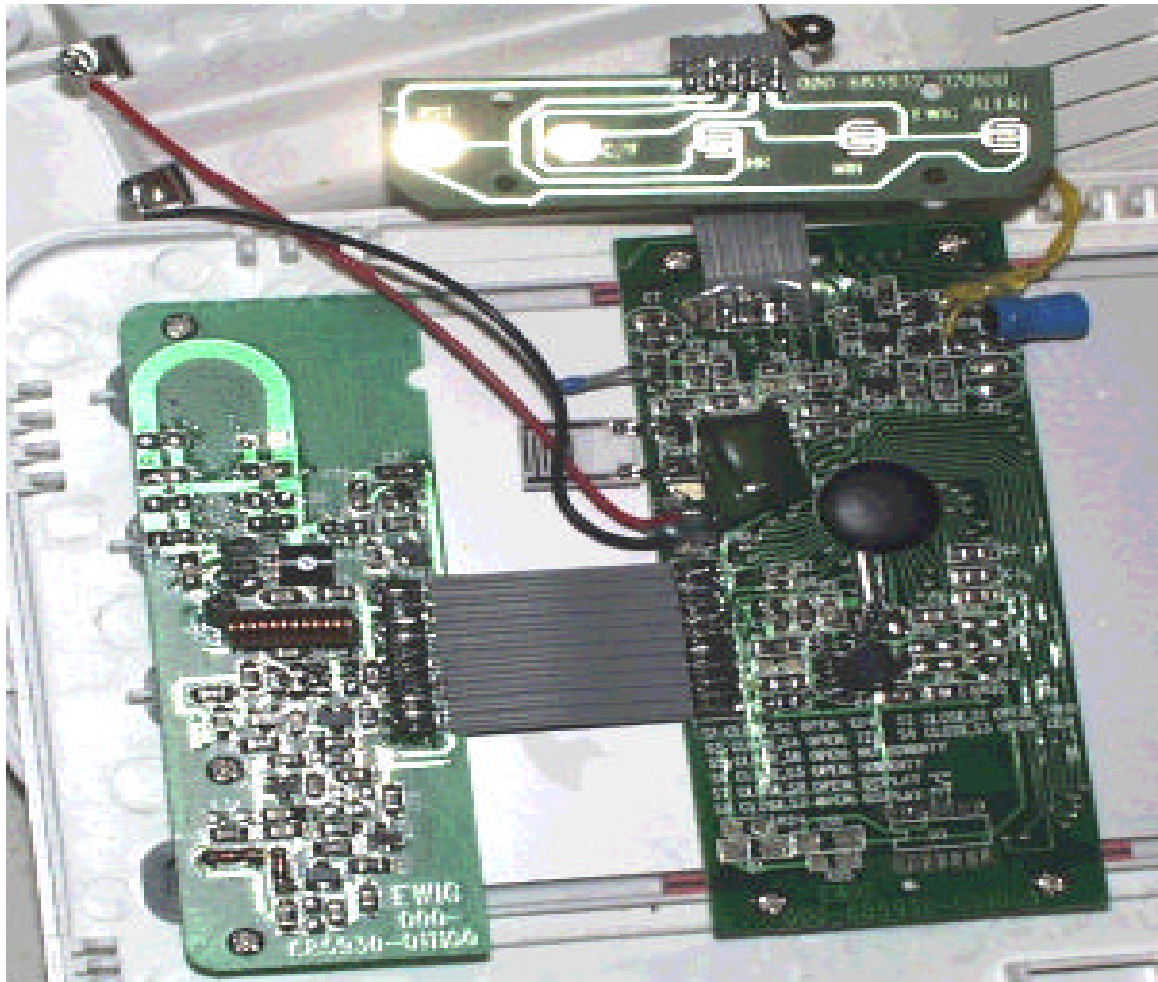
FCC ID: N9Z358F11 Real View of the Printed Wiring Board
