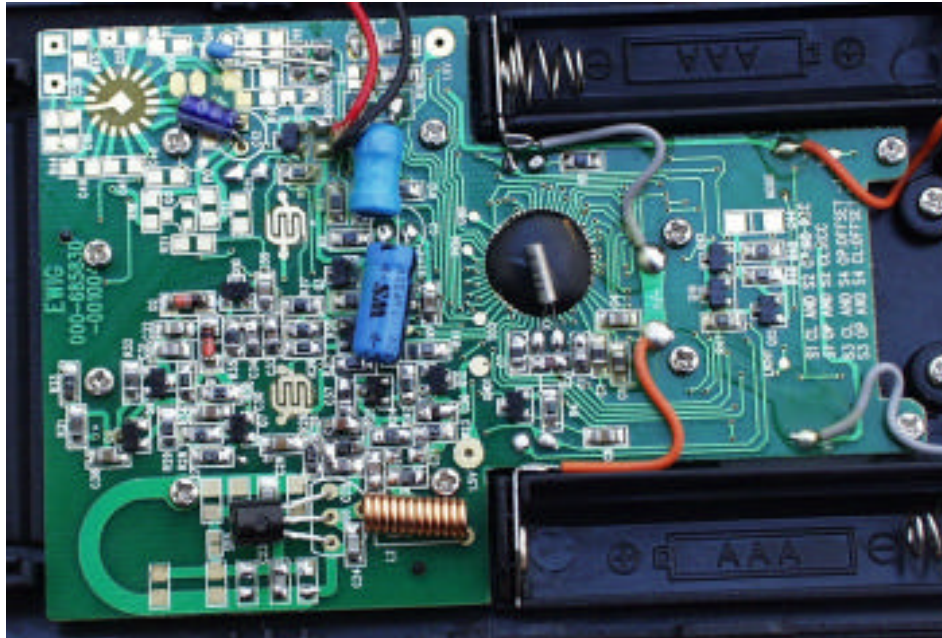
FRONT VIEW OF THE PRINTED WIRING BOARD
