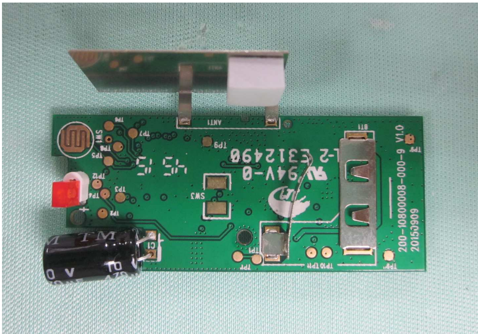
FCC ID: N9ZGRP008 PHOTOGRAPH OF THE PRODUCT
