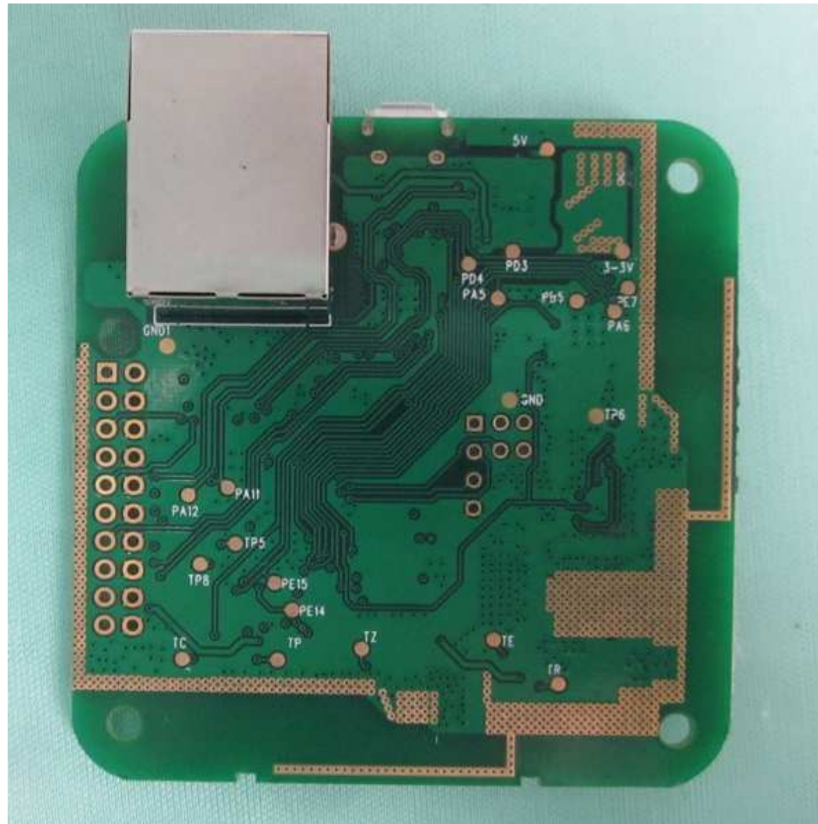
N9ZGRP009 PHOTOGRAPH OF THE PRODUCT INNER CIRCUIT BOTTOM VIEW
