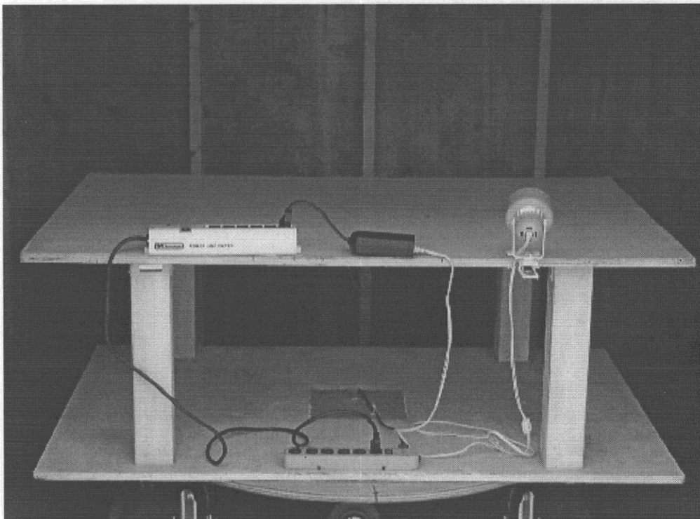
Figure 3.3 Radiated Rear
