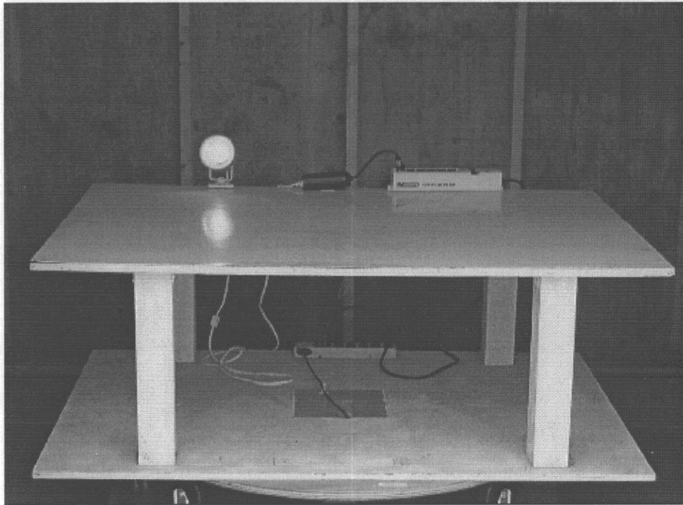
Figure 3.2 Radiated Front
