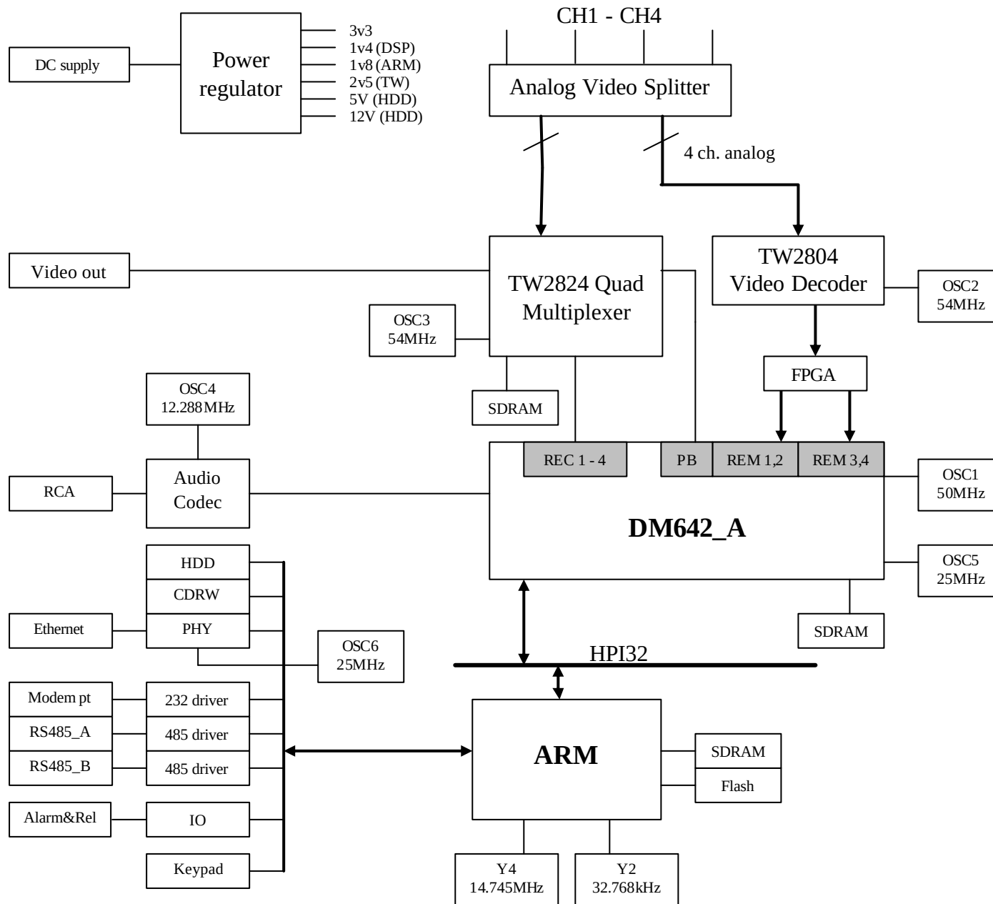
RX304 block diagram
