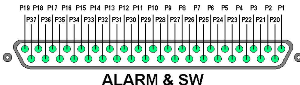
Pin assignment for TeleEye RX304
