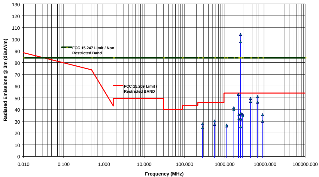
Transmitter Radiated Emissions Measurements at 3 Meter OFTS NETWAVE AIRSURFER PRO WLAN PC CARD, Model No.: 1100-6001 Channel #11: 2462 MHz, QPSK modulation with data @ 2 Mb/s
