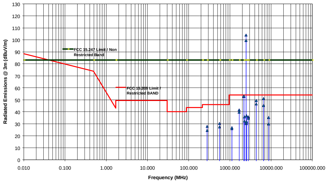
Transmitter Radiated Emissions Measurements at 3 Meter OFTS NETWAVE AIRSURFER PRO WLAN PC CARD, Model No.: 1100-6001 Channel #11: 2462 MHz, BPSK modulation with data @ 1 Mb/s
