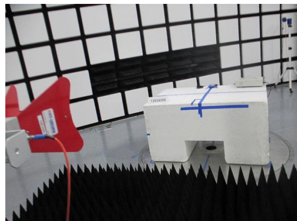
RADIATED FRONT PHOTO (1-18 GHz)
