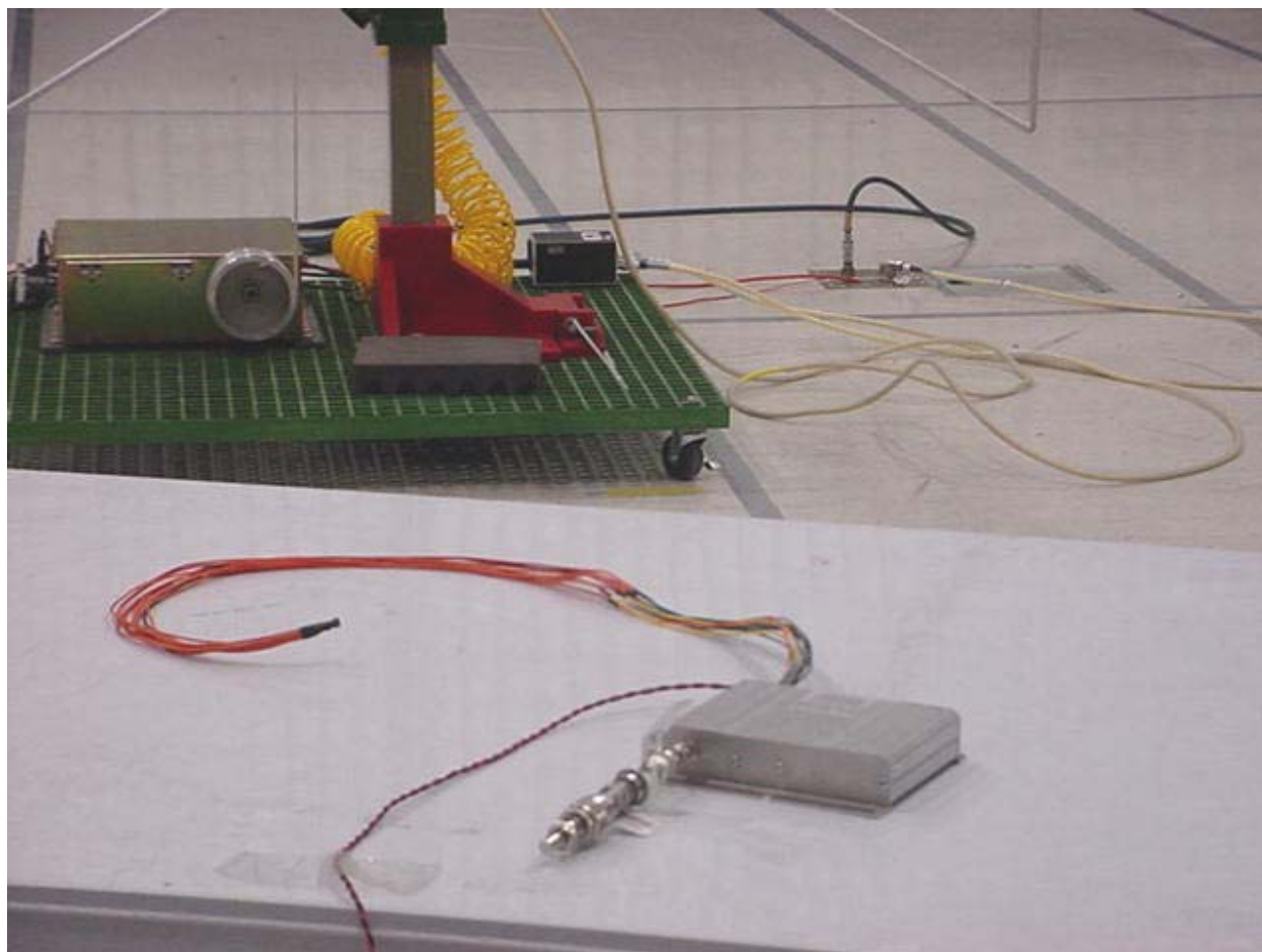
Spurious Radiated Emissions
