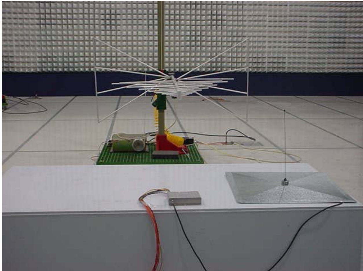
Radiated Emission from Digital Parts and Receiver
