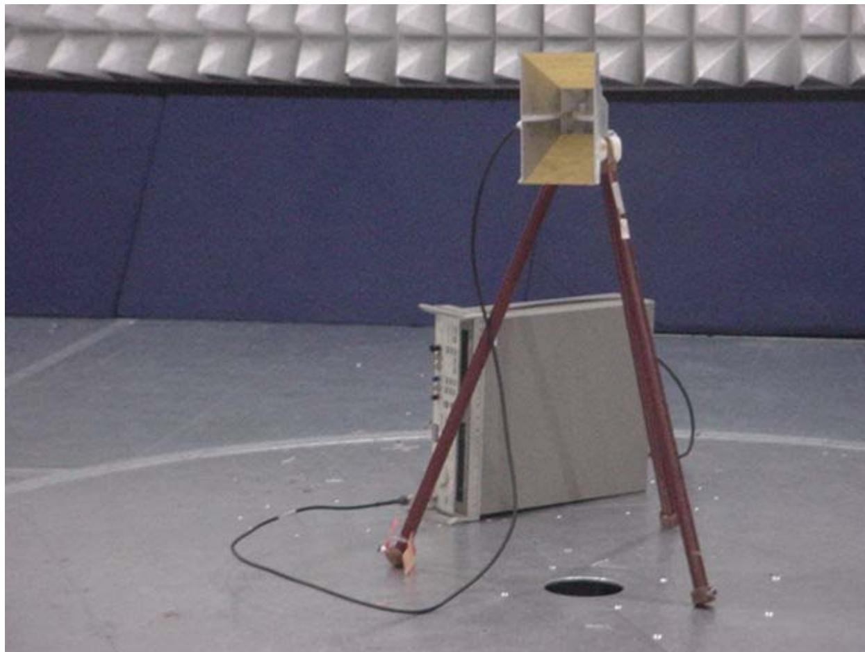
Spurious Radiated Emissions Substitution Method
