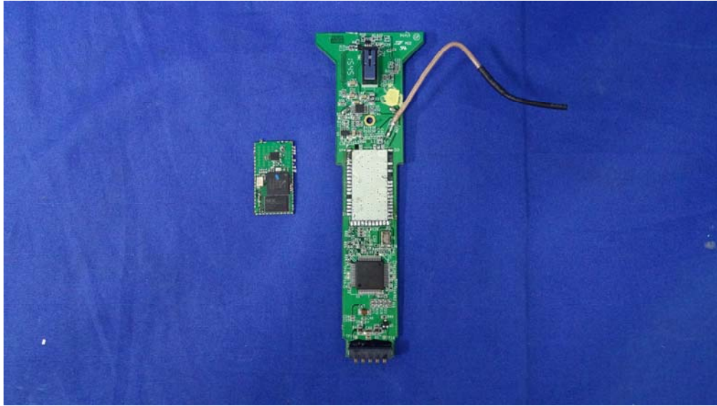
(7) EUT Photo
