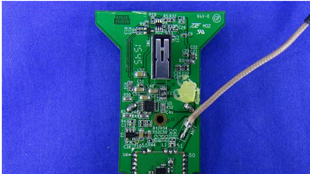
(11) EUT Photo
