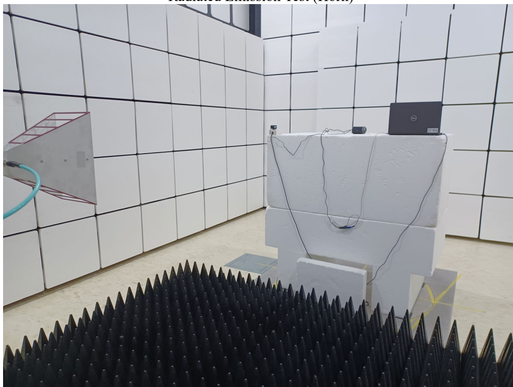
Radiated Emission Test (Horn)
