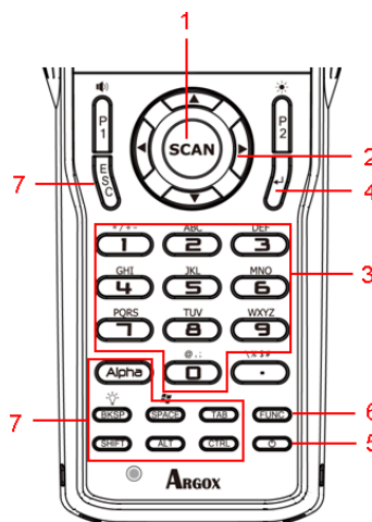
Figure 3-1 Keypad Description
