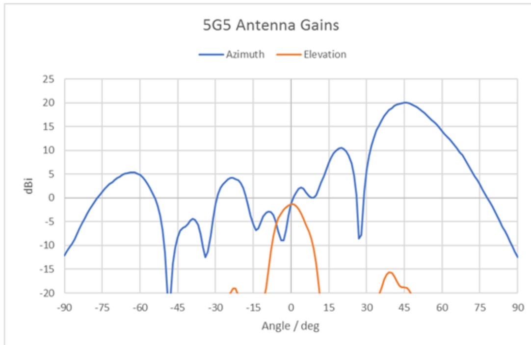
Fig. 2: Top: Antenna characteristics in azimuth and in elevation for Tx1. Bottom: Antenna characteristics in elevation@azimut=45° for Tx1. The peak gain is approx. 20 dBi.
