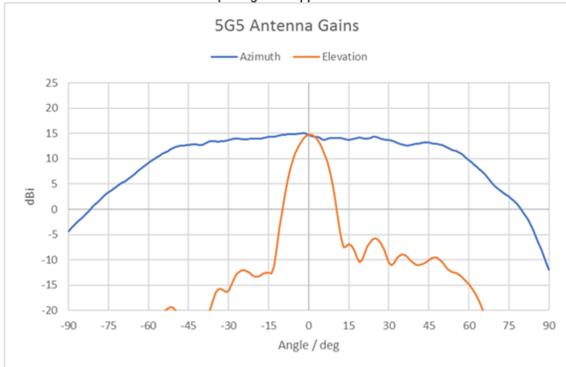
Fig. 3: Antenna characteristics in azimuth and in elevation for Tx2, Tx3 and receive antennas. The peak gain is approx. 15 dBi.
