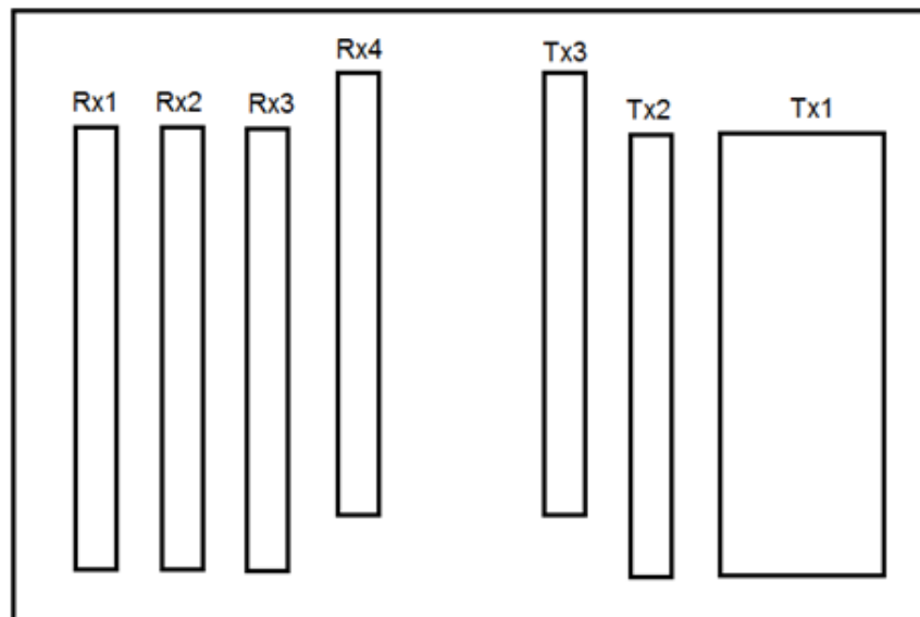
Fig 1: Illustration of Tx and Rx antennas inside the EUT. Each antenna consists of a patch array. The connector is located on the left side.
