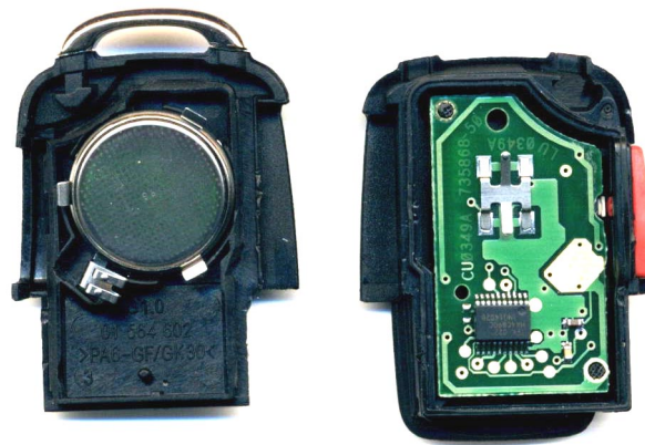
Photograph 10.3: Model 5FA 008 399-30: Internal view
