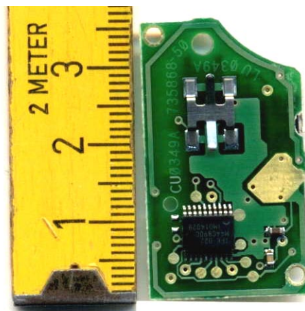
Photograph 10.4: Model 5FA 008 399-30: Internal view, PCB side 1
