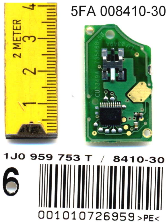
Photograph 10.10: Model 5FA 008 410-30: Internal view, PCB side 2
