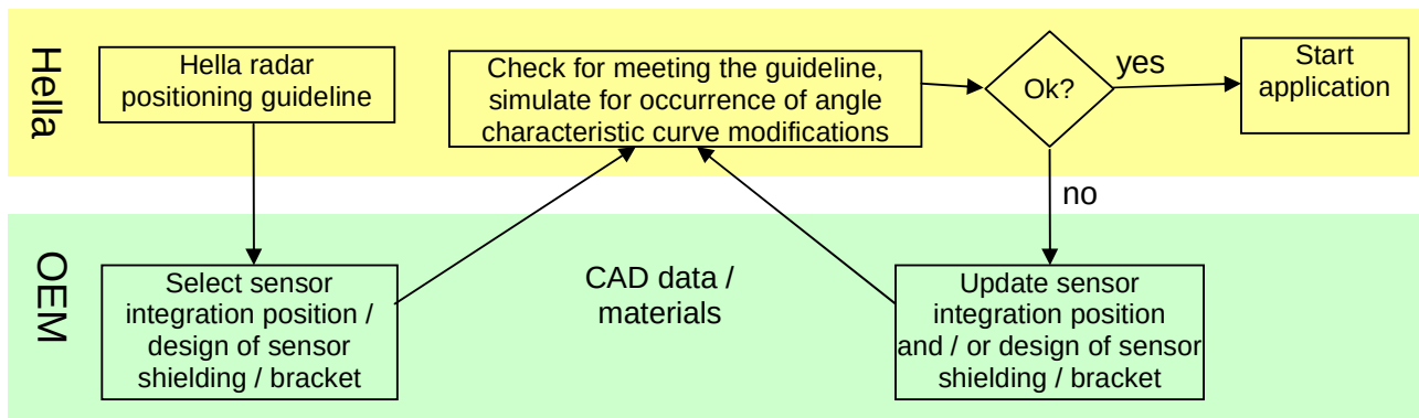
Fig. 1: Typical flow of the coordination process for the SBZA/LCA positioning.
