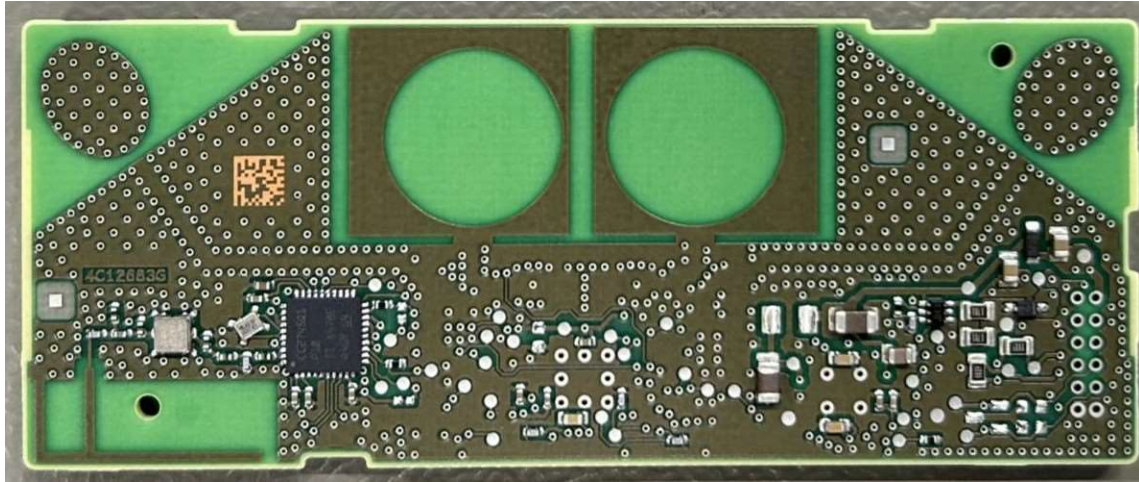
Picture 7: FBD6 PCB bottom photo
