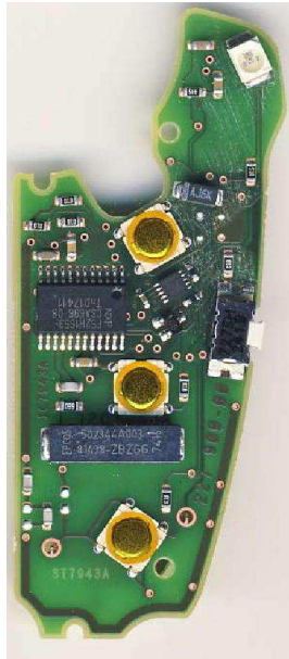
Picture 1: FS1271M PCB top
