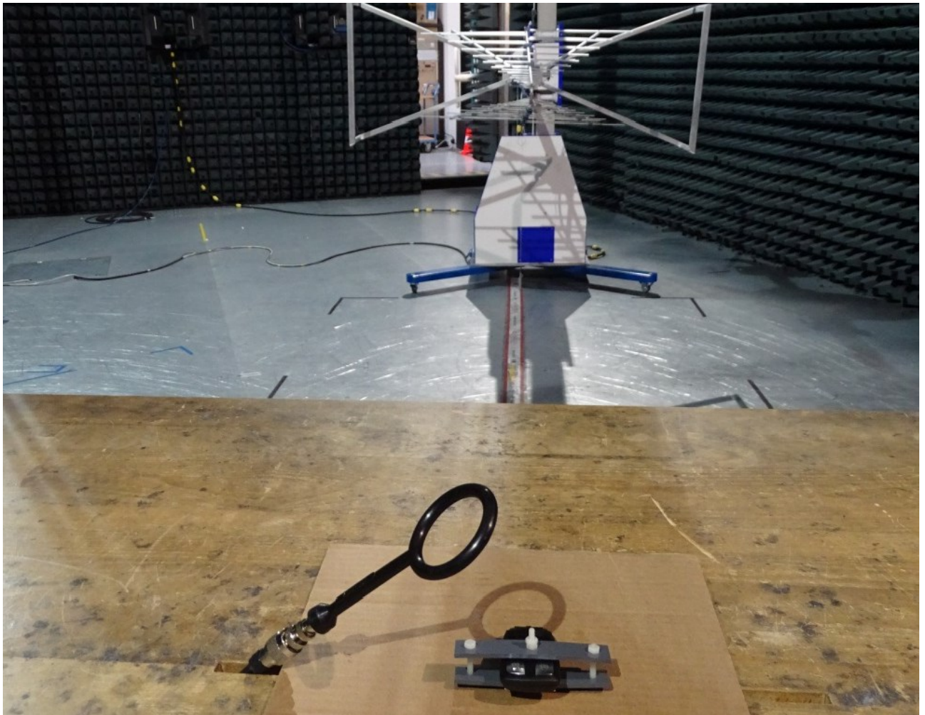
Photo 2: Test setup for radiated measurements (Enclosure, semi-anechoic chamber, 30 MHz to 1 GHz, intentional radiator §15, ANSI C63.10)
