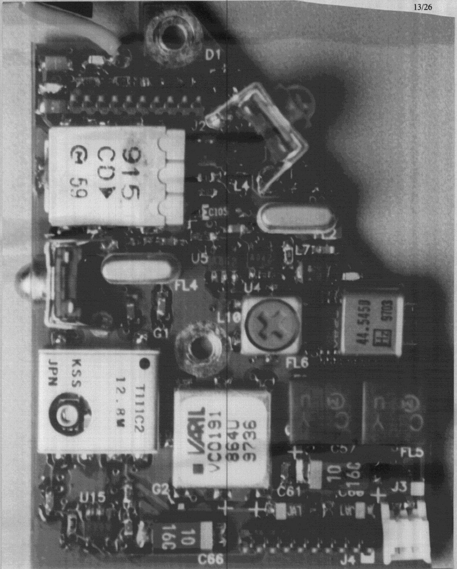
Photo 6: RF Board, Outside of Enclosure, PAD-1000
