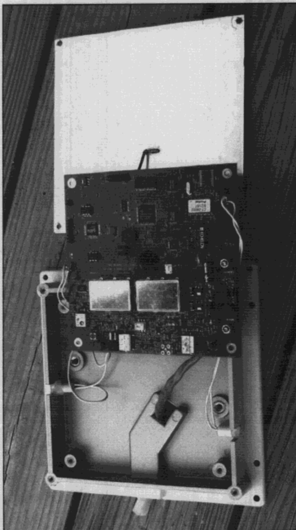
Photo 8: PROX-100, Horizontal, Wall Mount, Exploded View
