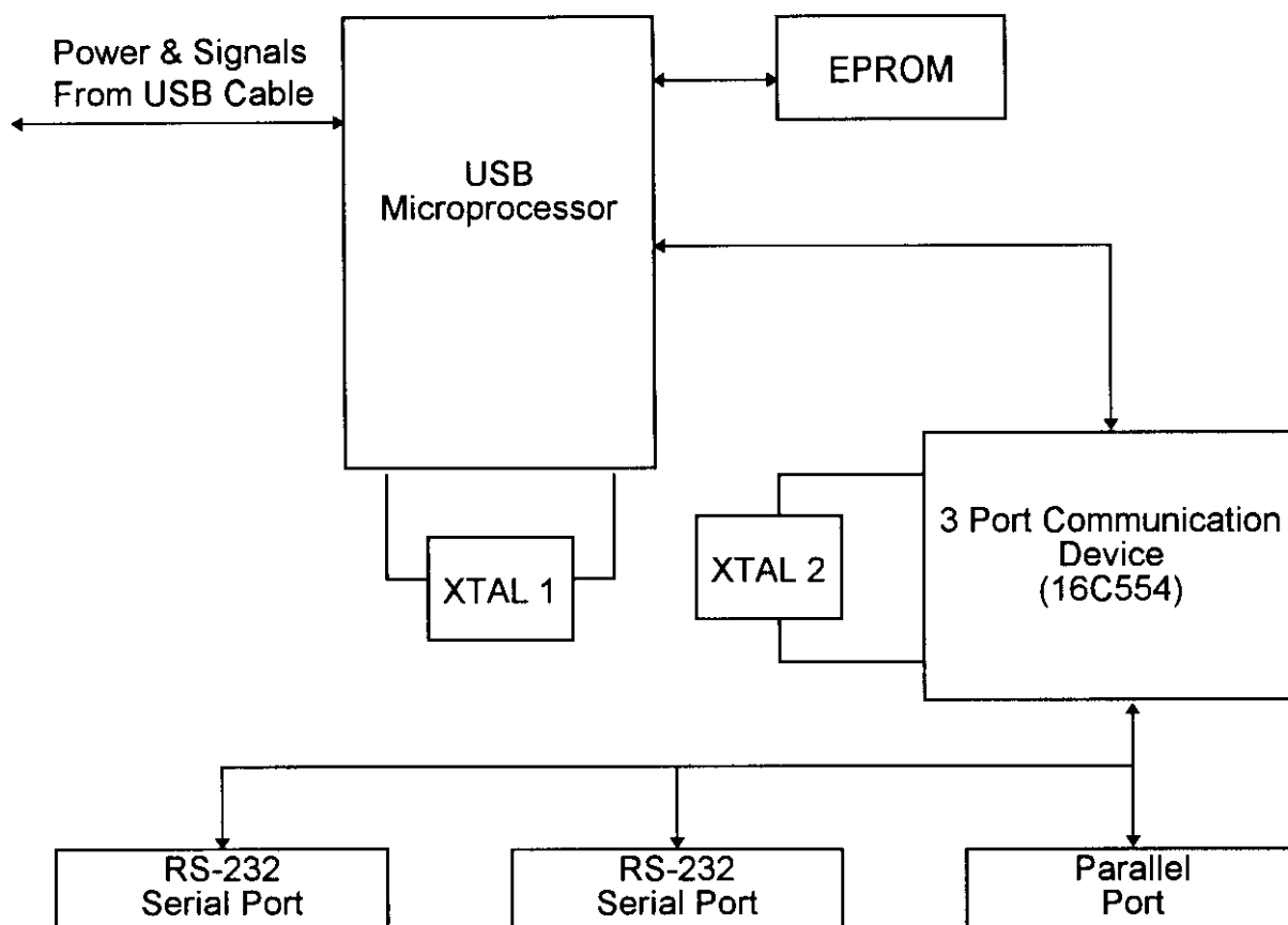
Figure 4.1 Block Diagram of EUT
